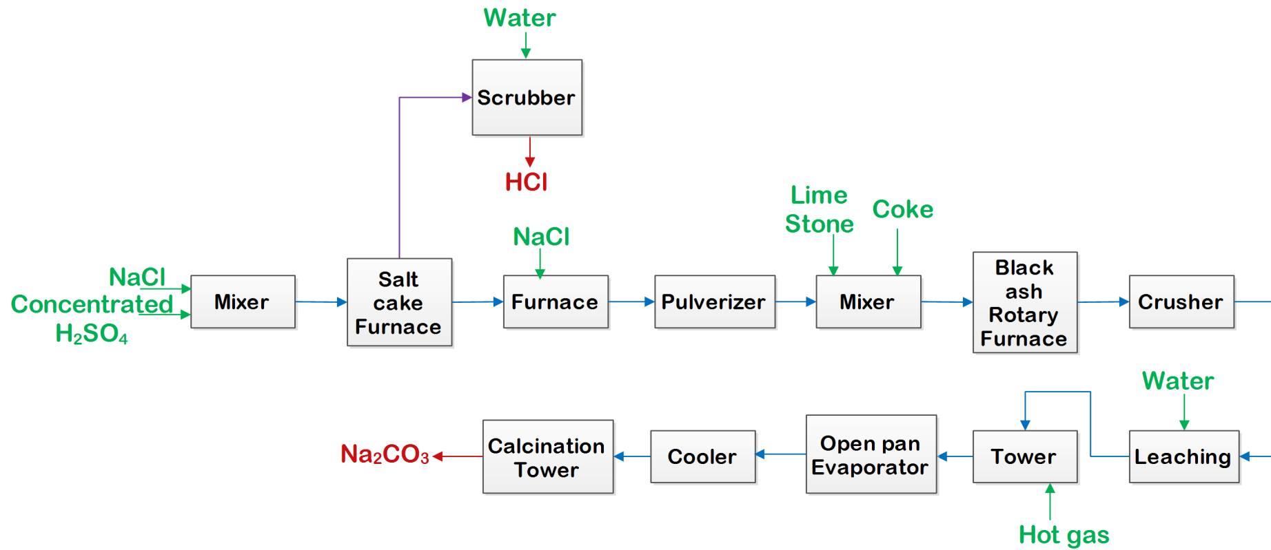
Figure: Manufacturing of Sodium Carbonate by Lablance process
